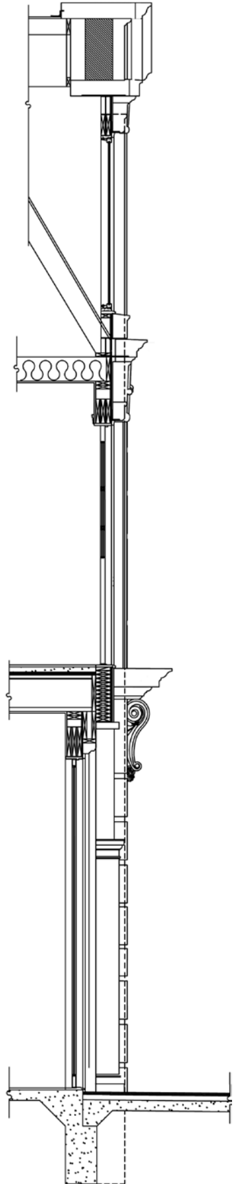
Front Facade Complete Drawing & Cross Section
